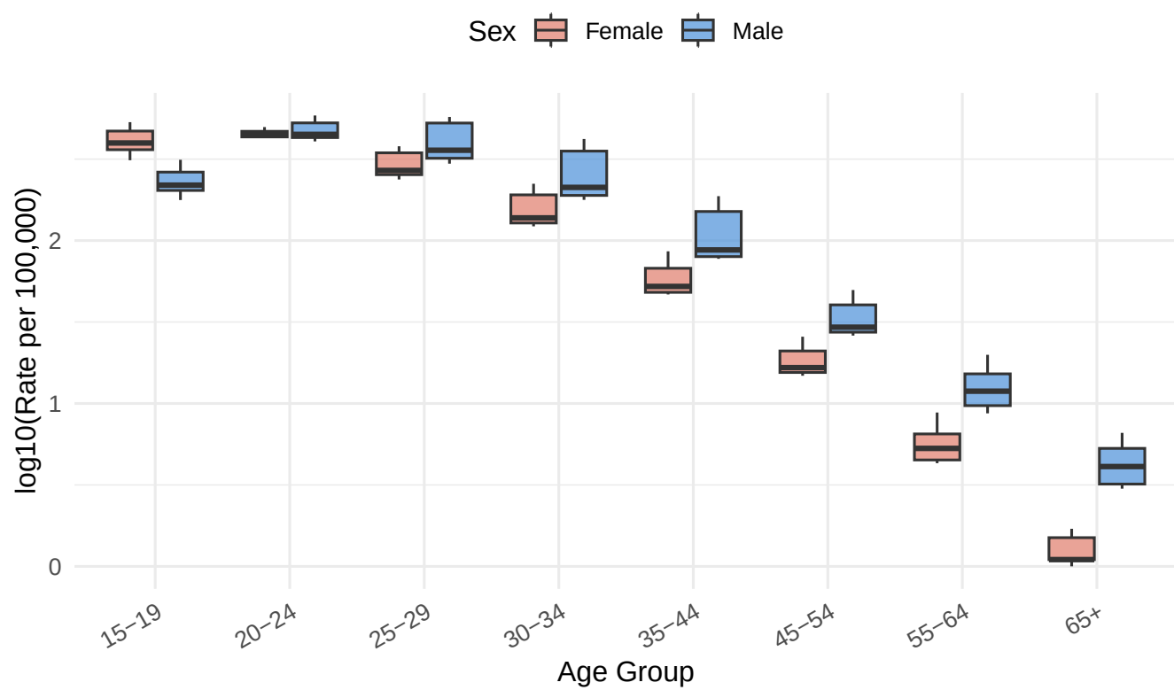
Figure 2: Distribution of log10-transformed gonorrhea rate by sex and age group.
